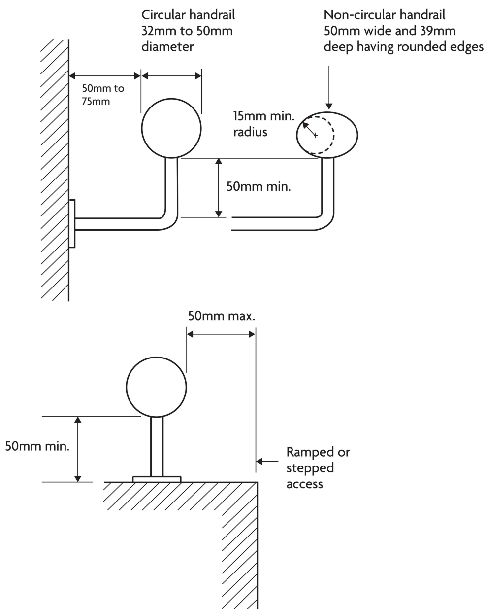
Diagram 1.13 Handrail design
